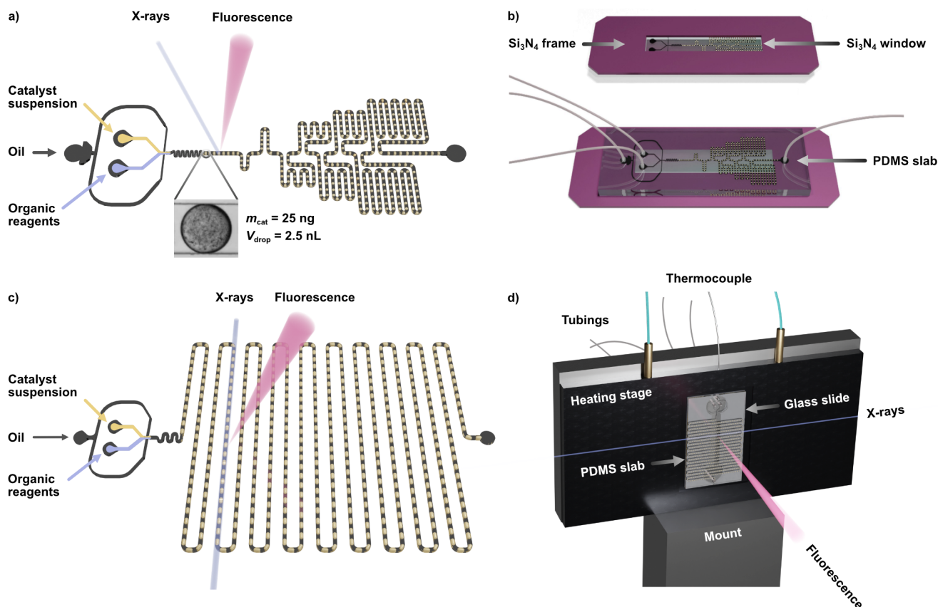
Figure 1. a) Scheme of the channel pattern and operational principle and b) bottom and top-view images of the L_3 -edge microfluidic device. c) Scheme of the channel pattern and operation principle and d) front view of the K -edge microfluidic device.
