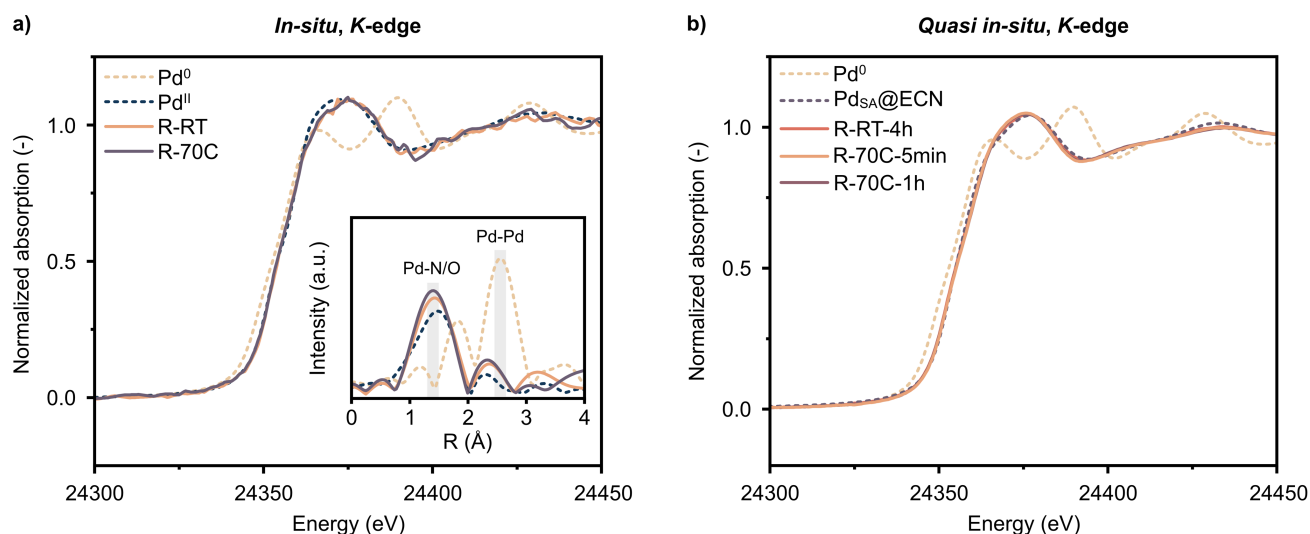
Figure 3. a) In-situ Pd K-edge XANES spectra of Pd SA @ECN under full reaction conditions, acquired at room temperature and at 70°C. Inset displays the corresponding FT-EXAFS spectra. b) Quasi in-situ K-edge XANES spectra of Pd SA @ECN under full reaction conditions, acquired at room temperature (R-RT-4h) and at 70°C (R-70C-5min, R-70C-1h). Corresponding conversions are provided in Table S3 .
