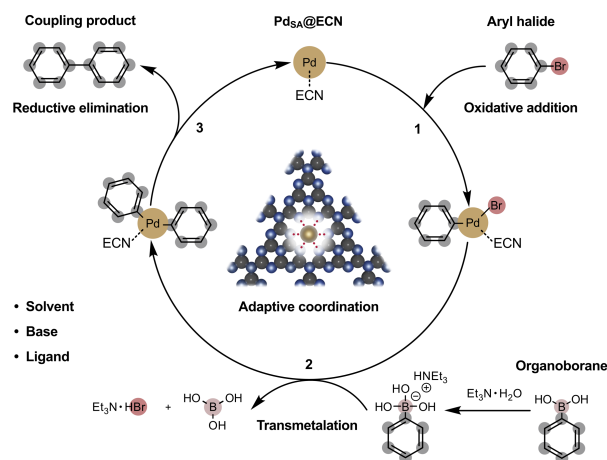
Scheme 1. Previously proposed Suzuki-Miyaura coupling mechanism over a \text{Pd}_{\text{SA}}@\text{ECN} catalyst, resembling the classical cycle over metal complexes. [7] The adaptive coordination of the catalyst during reaction lacks experimental verification.
