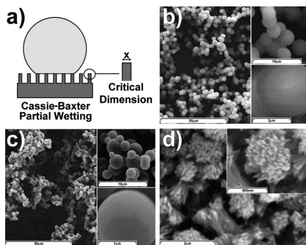
Fig. 1 (a) Diagram showing Cassie–Baxter superhydrophobicity and the critical dimension used to define surfaces here. Electron micrographs of (b) the larger scale sol–gel material, (c) the smaller scale sol–gel and (d) the copper oxide nano-pillars.
